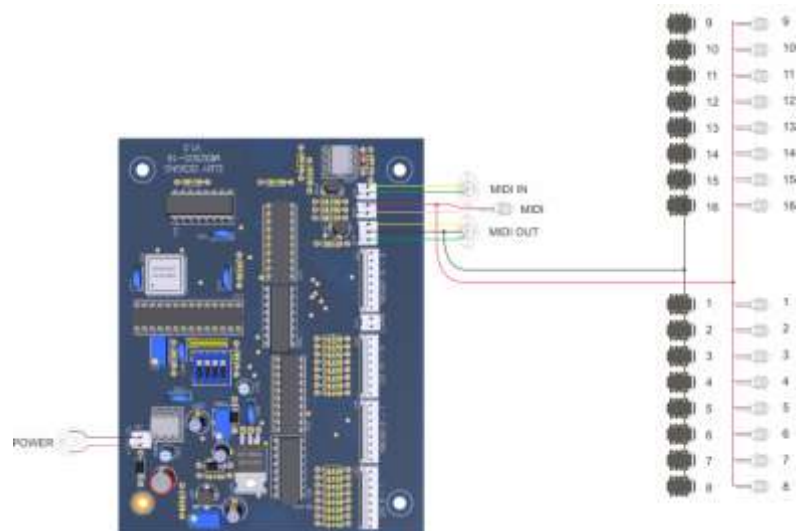
Figure 1 : Power and MIDI wiring – click for larger image
