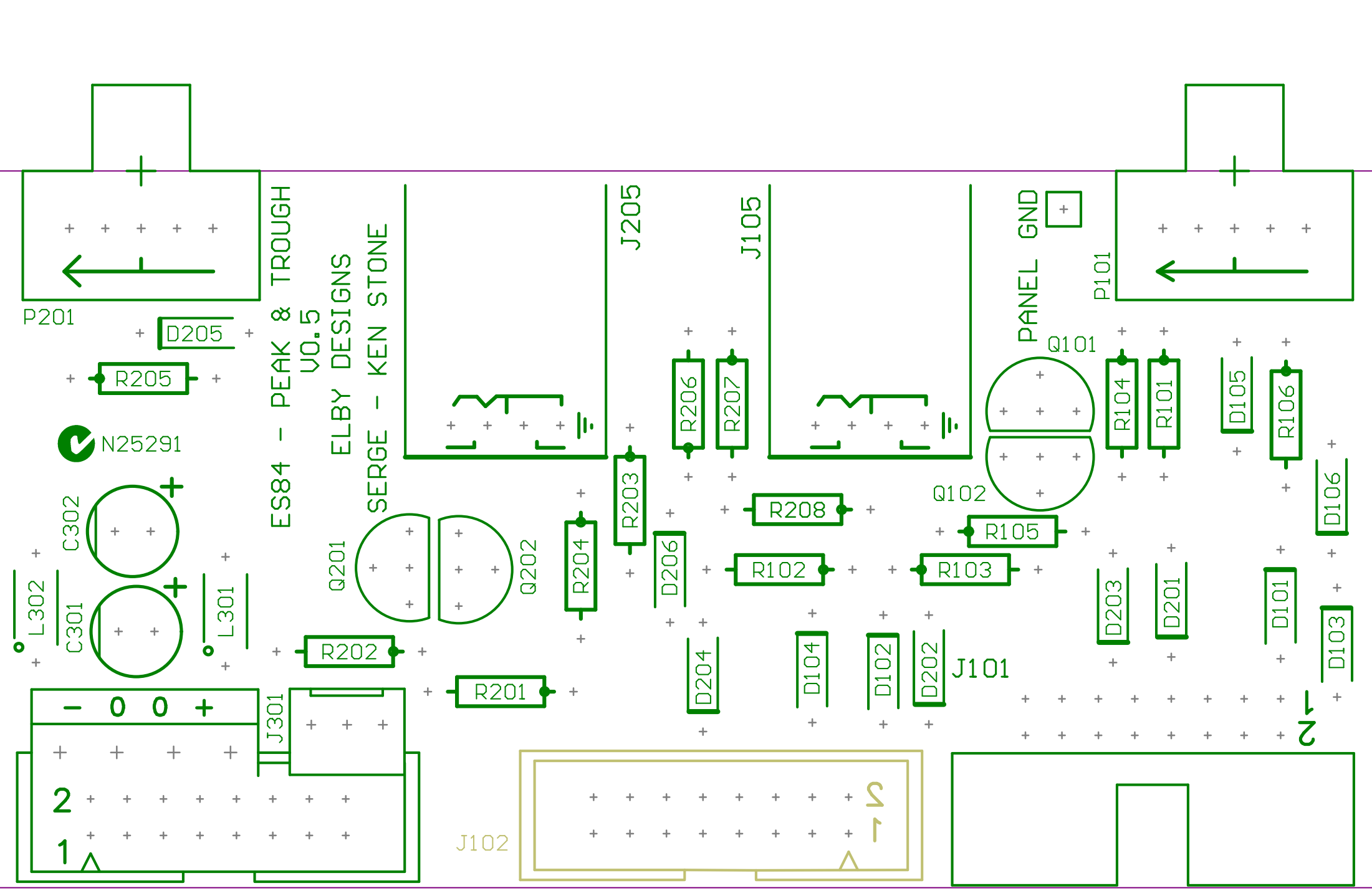
Column 3 PCB Overlay
