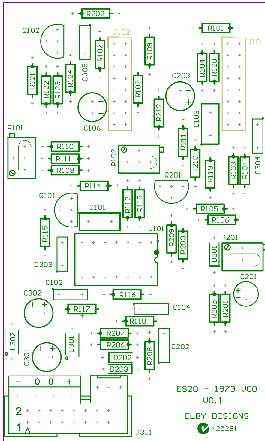
Backboard PCB Overlay
