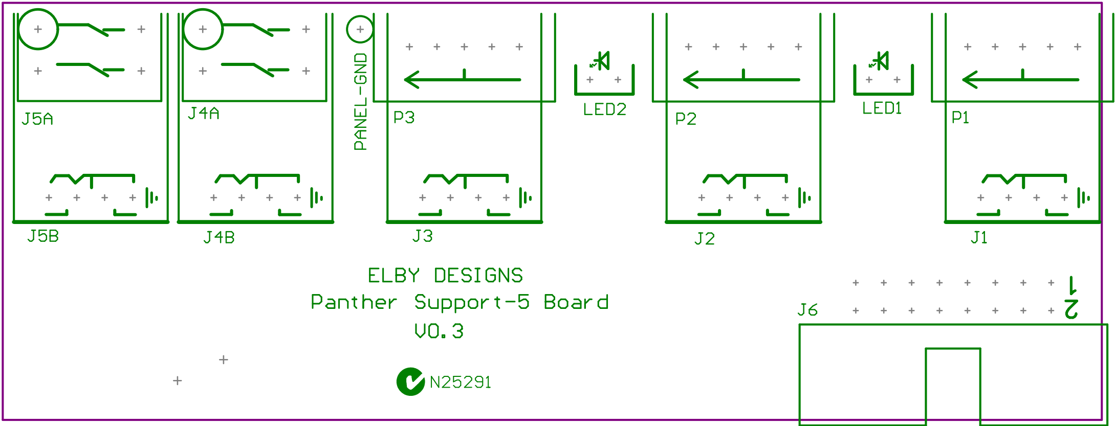
Column 1 PCB Overlay
