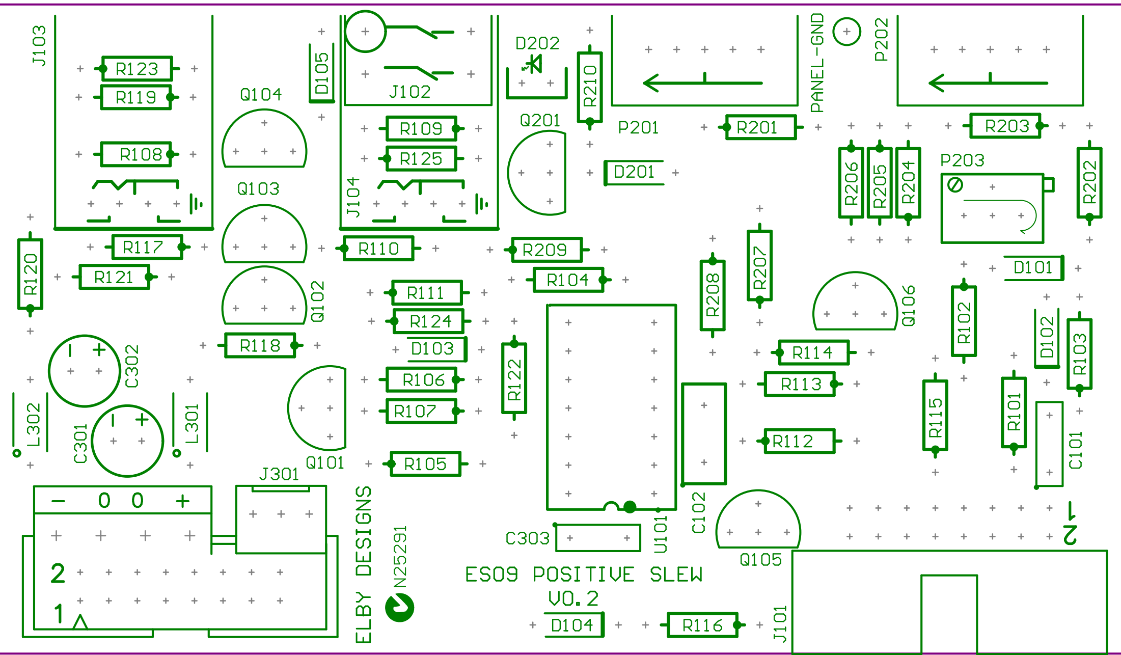
Column 2 PCB Overlay
