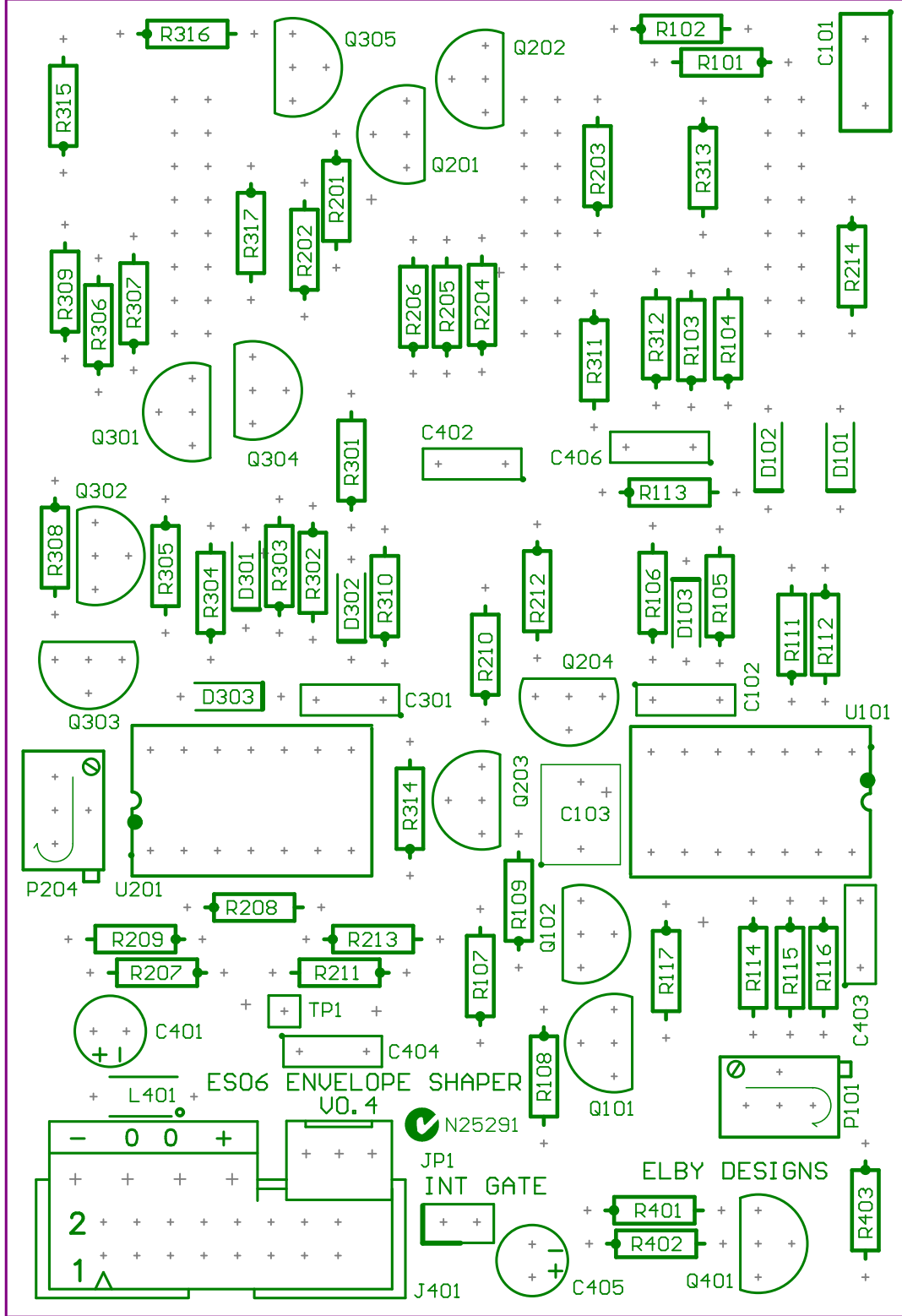
Backboard PCB Overlay
