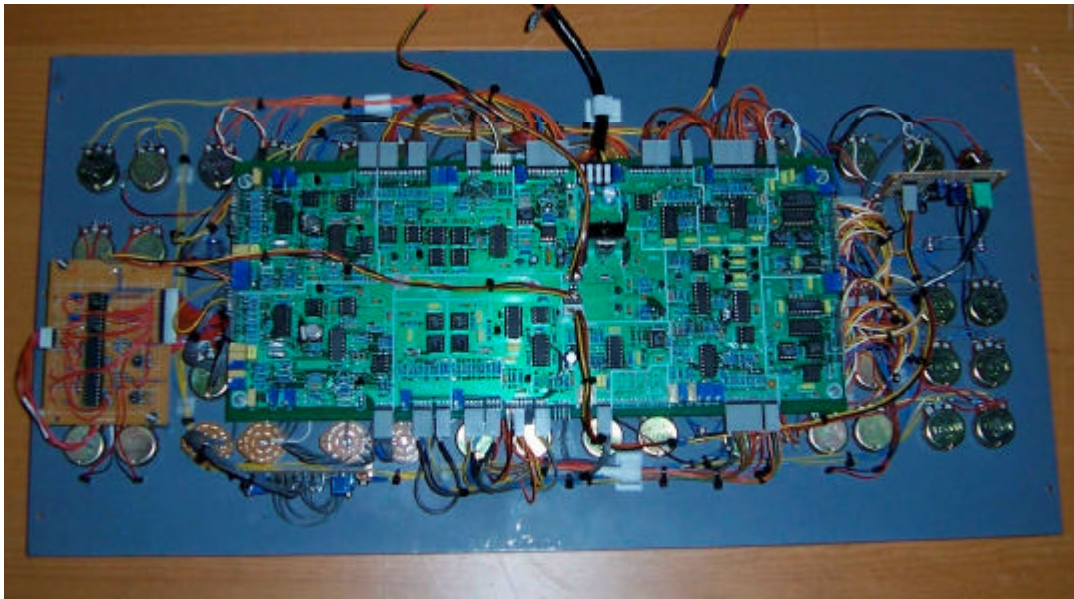
The ASM-2 and supporting circuits mounted to the rear of the front panel.
