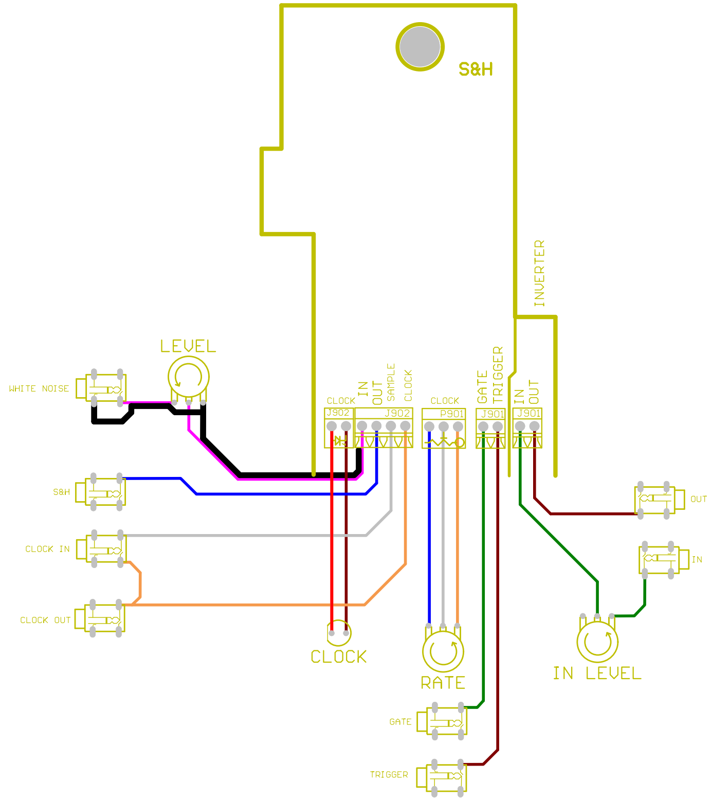
Panel components viewed from solder side
