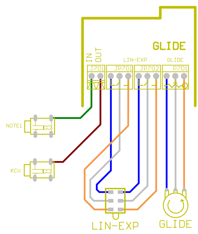
Panel components viewed from solder side
